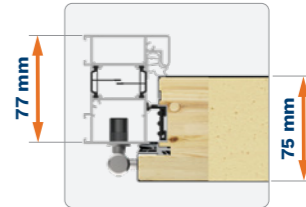
ALUTHERM 75 aluminium frame
