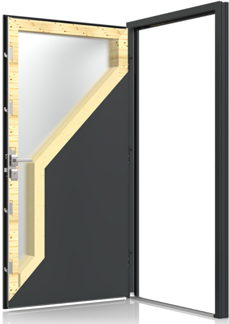
Adjustable keep enables smooth adjustment of the contact force of door and seals
